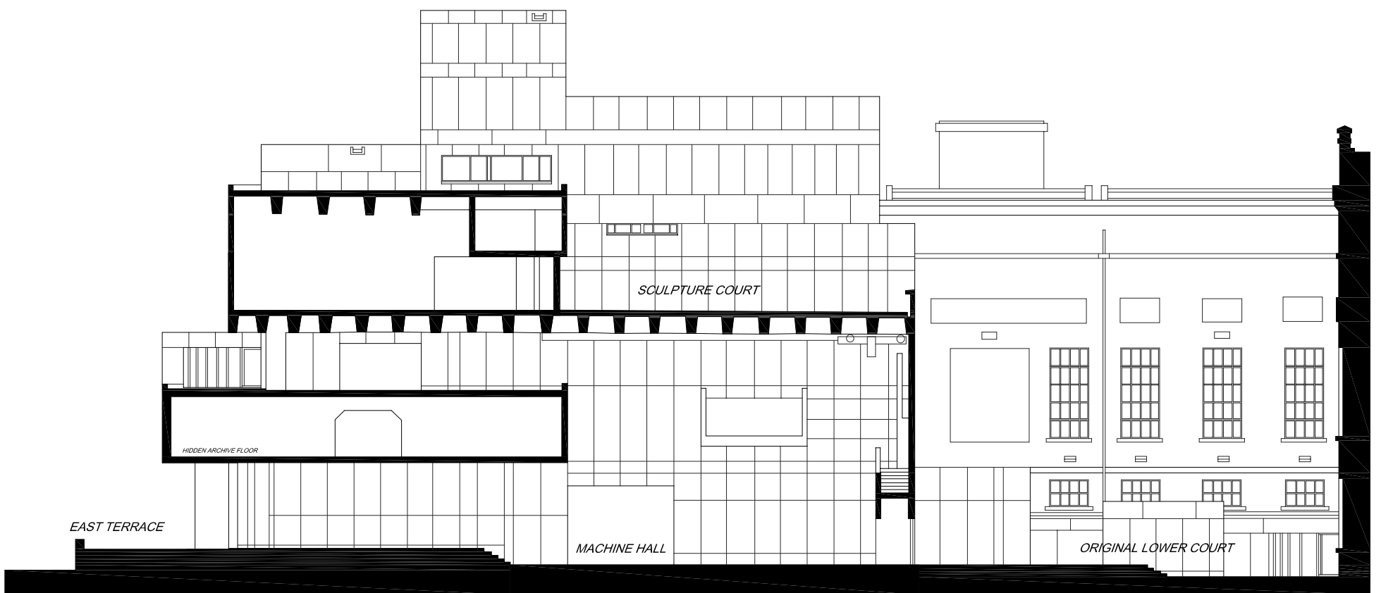
EXISTING SECTIONS
